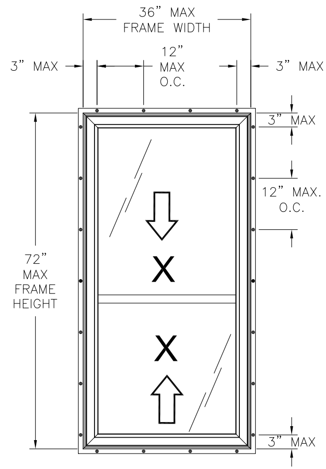
S-SERIES ORIEL DOUBLE HUNG EXTERIOR VIEW FIN INSTALLATION
