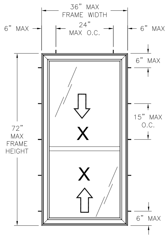
CAMBRIDGE ORIEL DOUBLE HUNG EXTERIOR VIEW FRAME INSTALLATION
